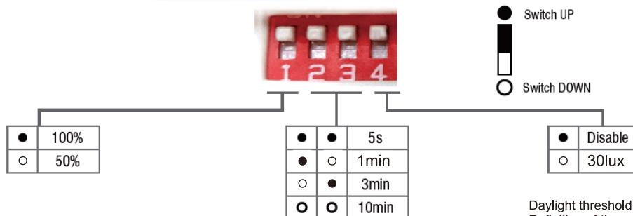
2 With insufficient ambient light, the sensor switches on the light when motion is detected.
