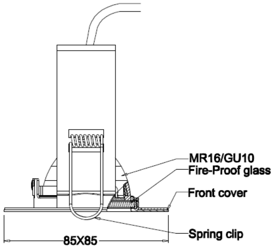
Figure 9 – Details of Downlighter Specimen G
