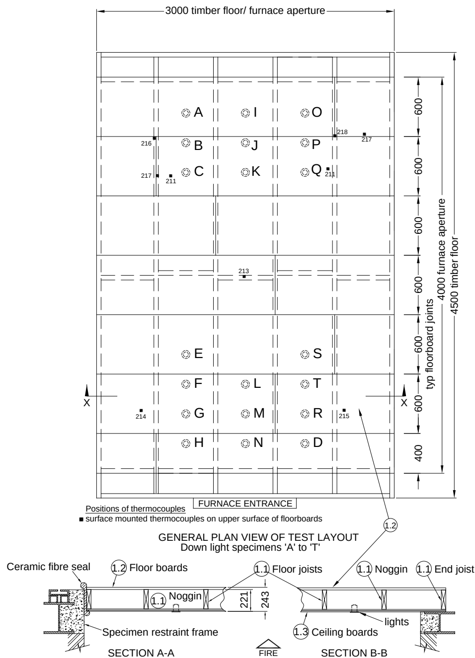
Figure 1- General Elevation of Test Specimens
