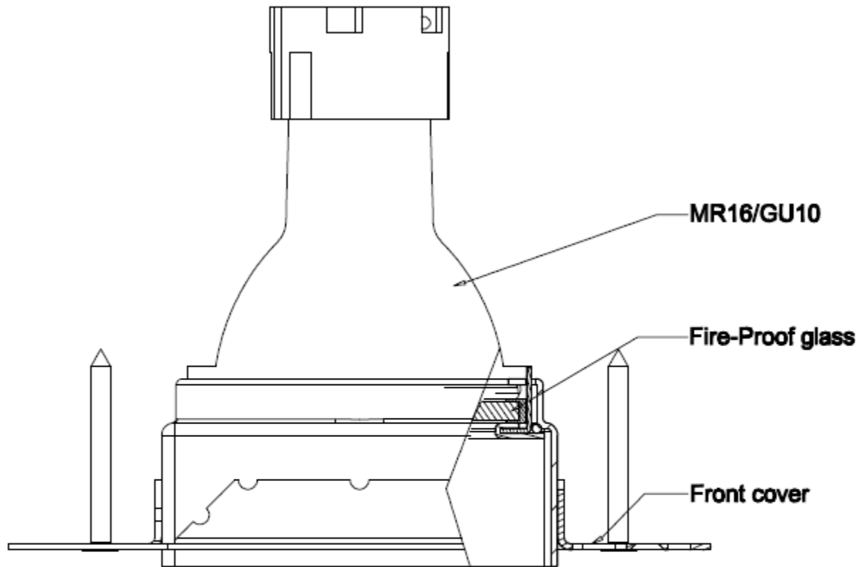
Figure 11 – Details of Downlighter Specimen I
