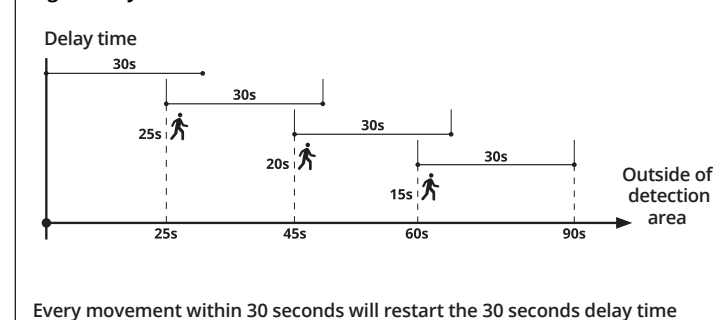
Fig. 2 Delay time within the detection area
